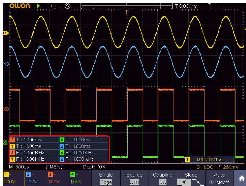
Figure 4-18 Automatic measurement
