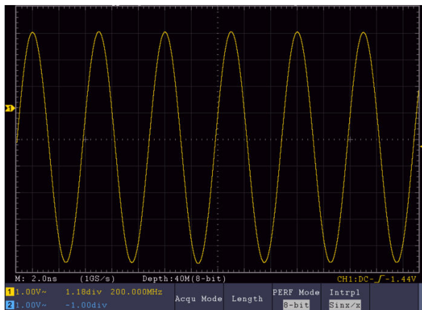
Sine(x)/x interpolation
