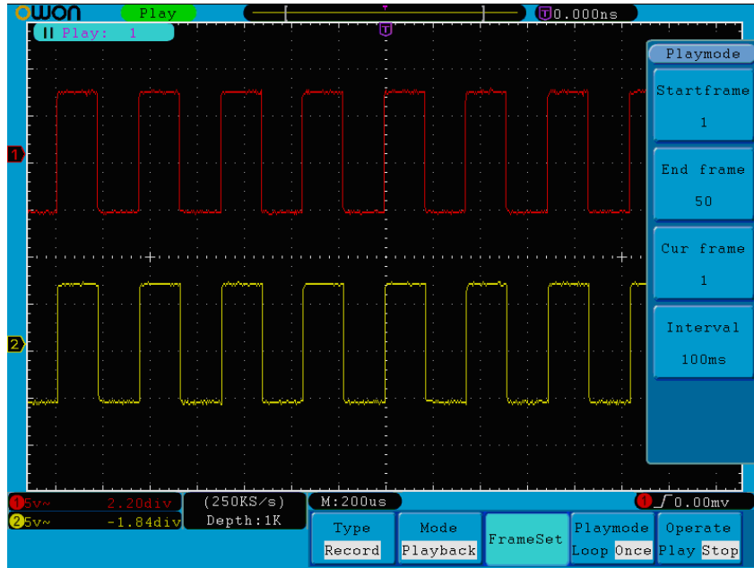
Figure 5-54 Wave Playback
