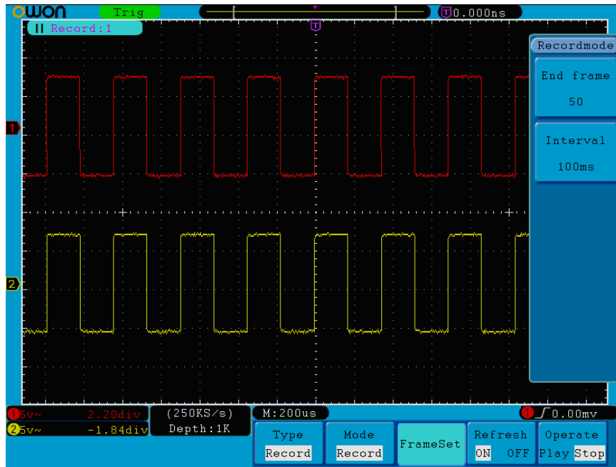
Figure 5-53 Wave Record
