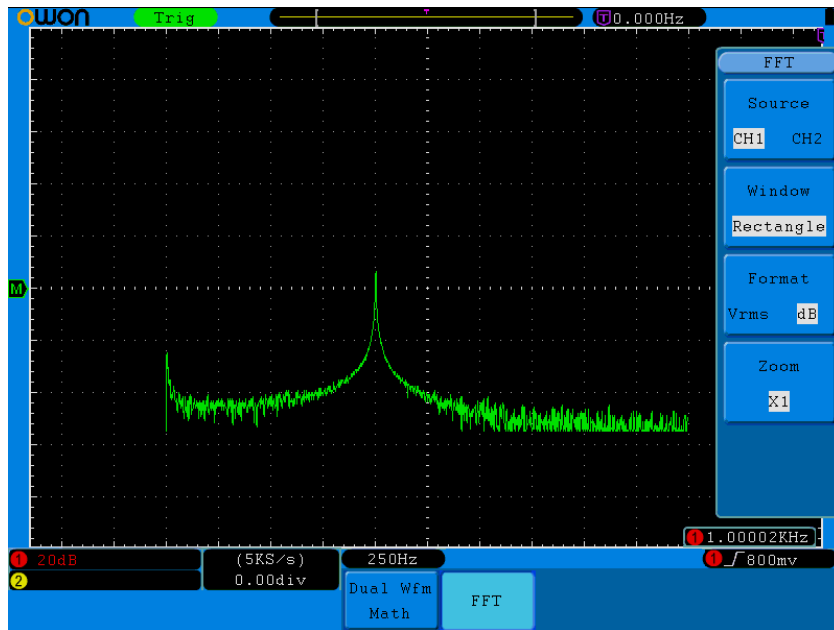
Figure 5-11 Rectangle window
