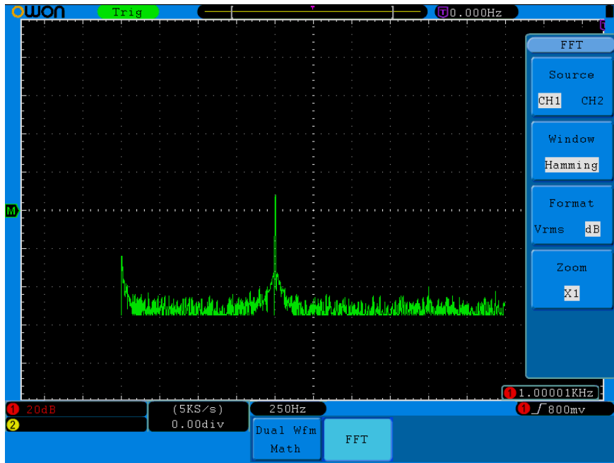
Figure 5-10 Hamming window
