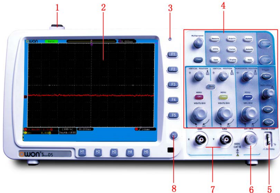
Figure 4-1 Front panel
