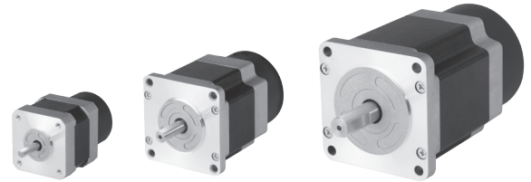
Frame size 42mm Brake built-in type 60mm Brake built-in type 85mm Brake built-in type
