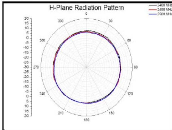
H Plane
